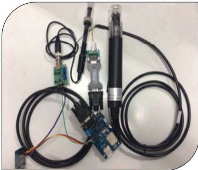
Fig. 4. Sensor measuring DO, Temperature & pH (Courtesy : Huan et al., 2020)
